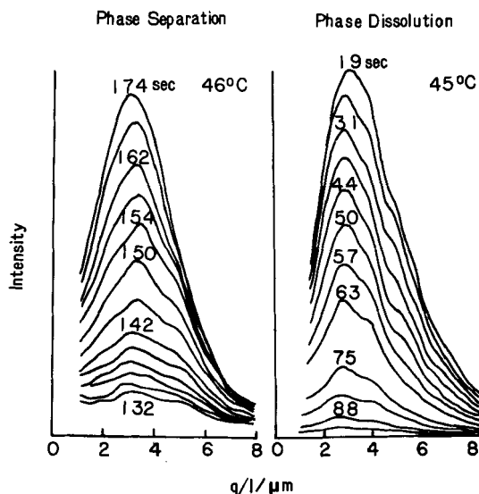
Figure 6. Time evolution of scattering curves of the 10 per cent aqueous HPC solution following a temperature jump from room temperature to 46^\circ\text{C} , and a reverse quenched from 46^\circ to 45^\circ\text{C} .
